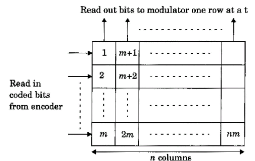
Fig. 17 Block interleaver where source bits are read into columns and
